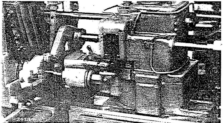
Fig. 17. Cam-operated closing arrangement for a rotating diehead on a Brown & Ward \frac{5}{8} " Automatic Screw Machine
