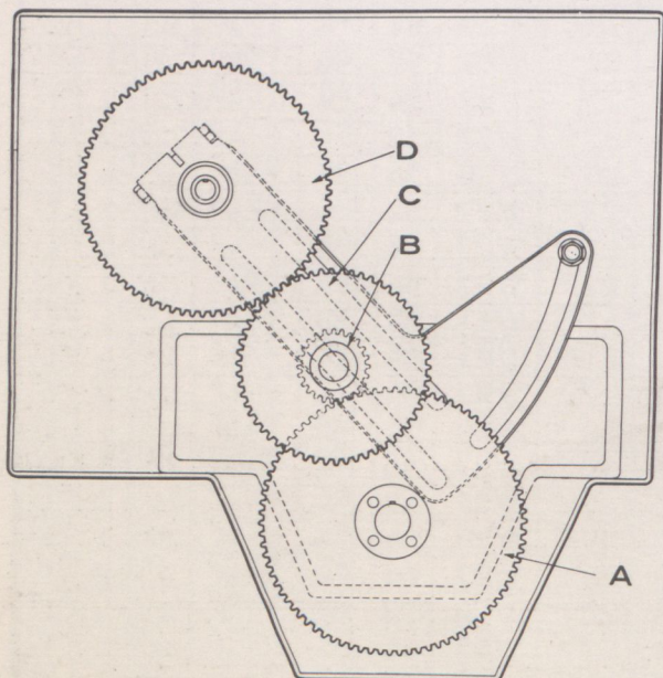
RIGHT HAND DIVIDING HEAD
