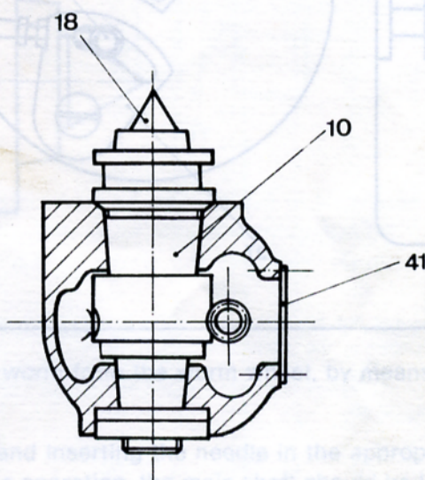
Vertical position of the dividing head
