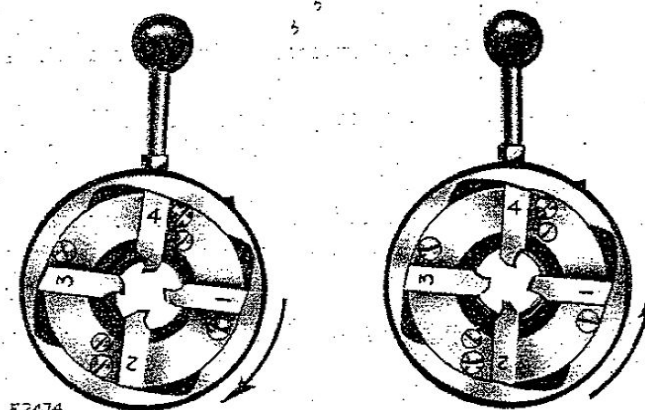
Fig. 25. The correct order for inserting dies. Arrows indicate the direction of work rotation.
