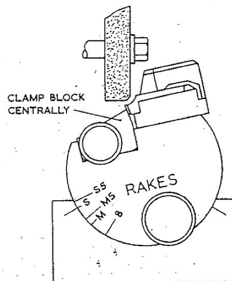
Fig. 67. The setting of S type dies
