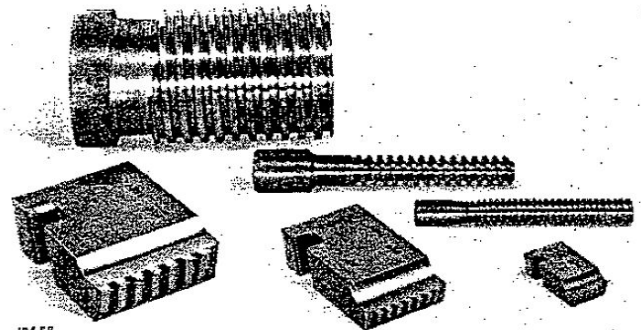
Fig. 36. Acme threads cut with Holozone dies. Shown are 1\frac{3}{4} \times 5 , \frac{3}{8} \times 8 and \frac{5}{16} \times 14 T.P.I. Excellent finish is obtained.
