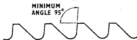
Fig. 44. Buttress Thread
