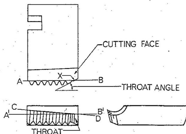
Fig. 49. Diagram to illustrate the cutting and self-guiding action of Coventry Dies
