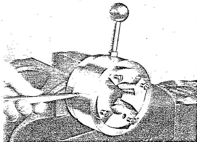
4. Remove the two screws which hold together the external and internal scroll.
