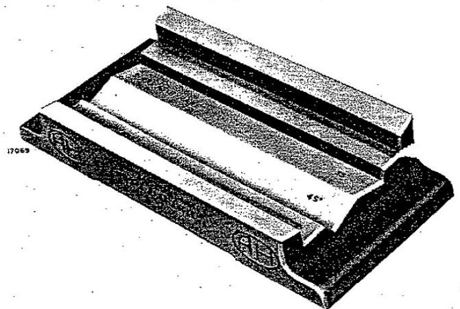
Fig. 51. The baseplate used when grinding 15°, 33° and 45° throat angles and 5° and 13° rake angles
