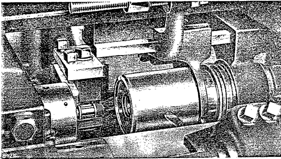
Fig. 19. Coventry Rotating Diehead on types F. & G. Gridley 4-spindle Automatics
