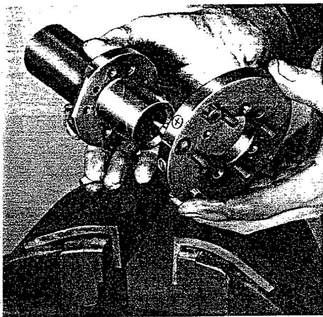
6. Insert the four cheese-head screws in the back-plate and assemble the plate on the shank.
