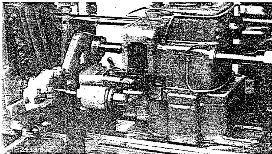
Fig. 17. Cam-operated closing arrangement for a rotating diehead on a Brown & Ward \frac{5}{8} " Automatic Screw Machine
