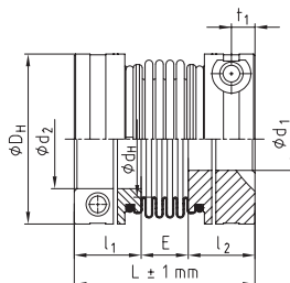
TOOLFLEX® Version S - 2.5
