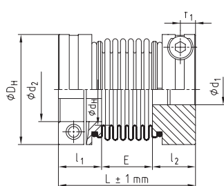
TOOLFLEX® Version M - 2.5
