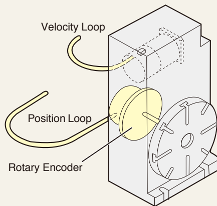
Configuration of High Precise Indexing Models
