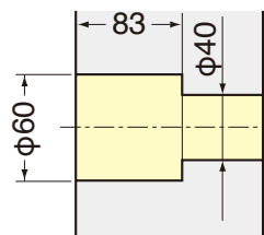
Face Plate Through Hole
