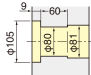
Face Plate Through Hole
