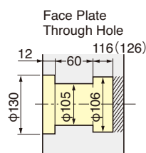
Clamp Device
