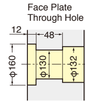
Clamp Device
