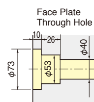
Clamp Device
