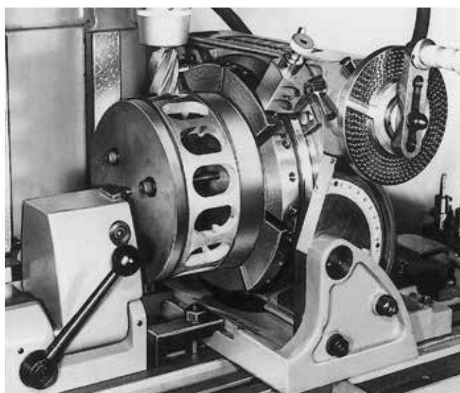
Vertical indexing operation
