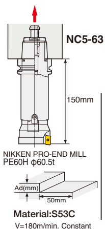
Comparison of Milling Capability using extended cutter
