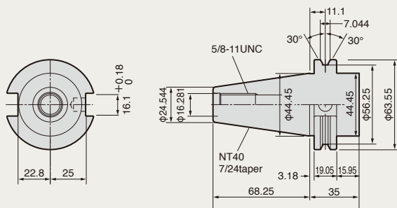
CAT40
