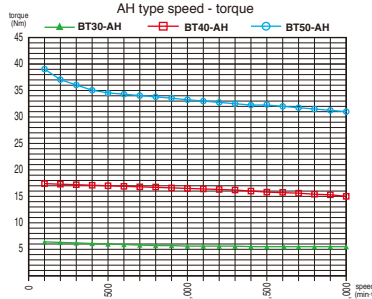
ANGULAR HEAD(AH) speed(min -1 )-torque(Nm)/power(kW)
