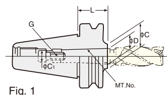
Draw bolt type
