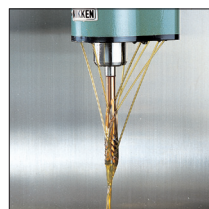
multi oil hole holder
