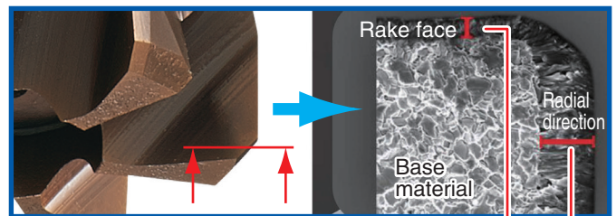
Non-uniform coating film thickness
