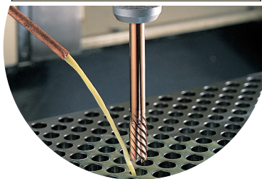
Photo shows NC Sensor Reamer NCS
