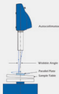
Rotary Table Calibration
