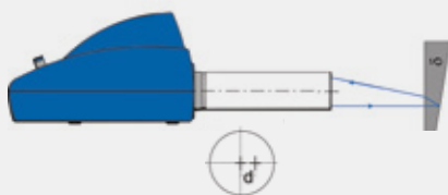
Wedge Angle Measurement in Reflection / Double Pass
