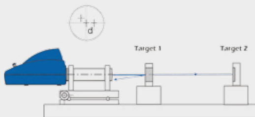
Alignment of Optical Components
