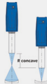
Measurement of Slightly Curved Surfaces
